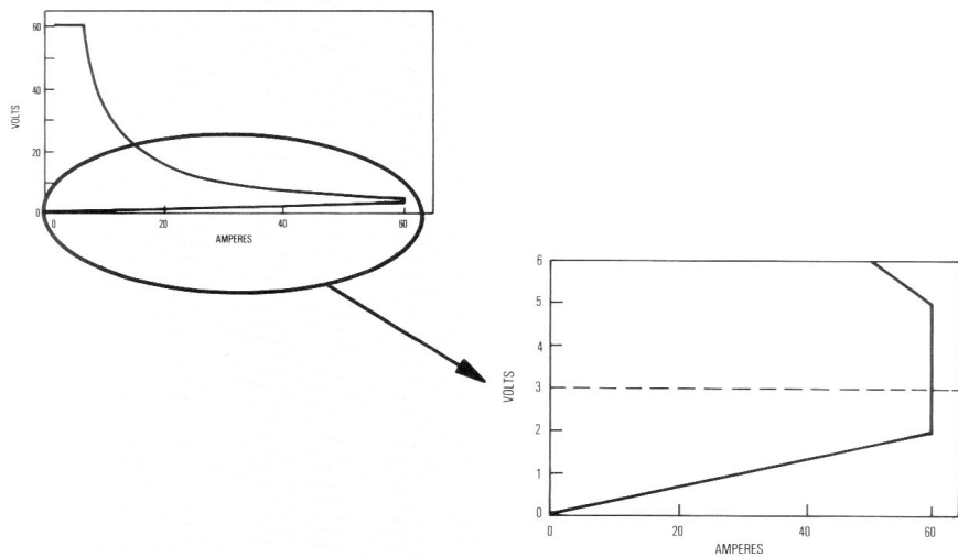
Figure 8. Operating Characteristics of an Agilent Electronic Load
